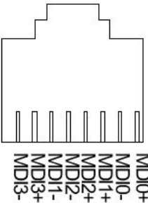
10/100/1000Base-Tx RJ-45 Connector
