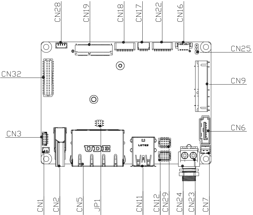
Top View
