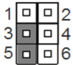
Clear CMOS
