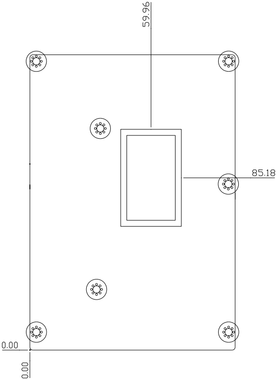
Solder Side
