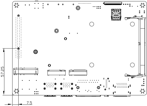
Solder Side
