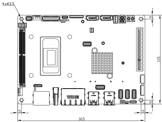
Component Side
