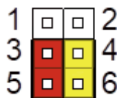
Pins 3-5 and 4-6 selected Non +5V_DUAL Power
