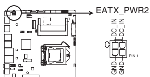
MIX-H310D1 1 x 4 PIN (2x2) internal power connector
