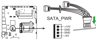
MIX-H310D1 SATA POWER connector
