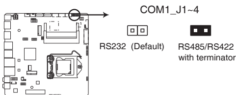
MIX-H310D1 COM1 RS422/RS485 Terminator (J1/J2/J3/J4)
