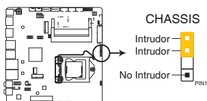
MIX-H310D1 Chassis intrusion connector
