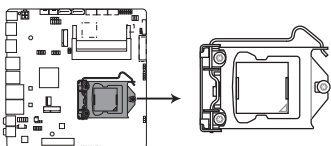
MIX-H310D1 CPU socket LGA1151
