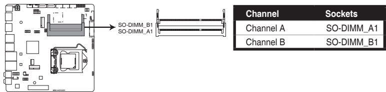
MIX-H310D1 240-pin DDR4 SO-DIMM sockets
