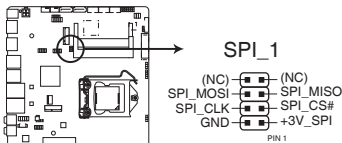
MIX-H310D1 BIOS Programmable connector
