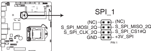
MIX-Q370D1 BIOS Programmable connector
