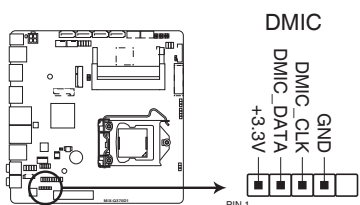
MIX-Q370D1 DMIC connector
