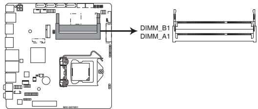
MIX-Q370D1 260-pin DDR4 DIMM sockets
