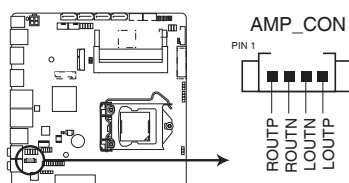
MIX-Q370D1 Audio stere. output with Amp connector
