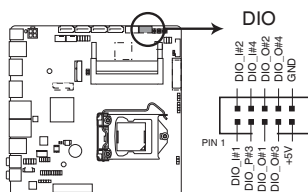
MIX-Q370D1 Digital I/O connector
