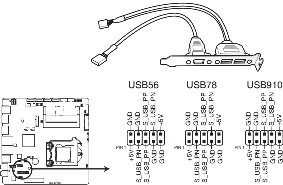
MIX-Q370D1 USB2.0 connectors
