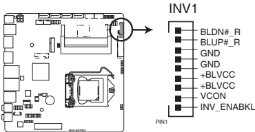
MIX-Q370D1 Inverter connector
