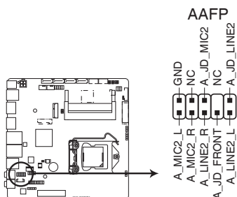
MIX-Q370D1 Front panel audio connector
