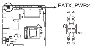
MIX-Q370D1 1 x 4-pin (2x2) internal power connector
