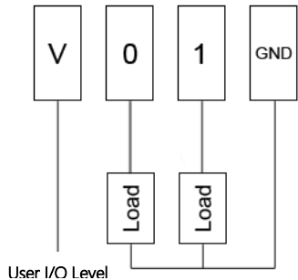
Wet Contact Wiring
