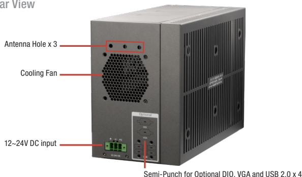
BOXER-6842M-A4
