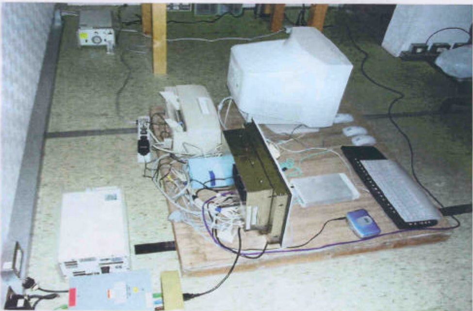
The Photograph of Conducted Susceptibility Test
