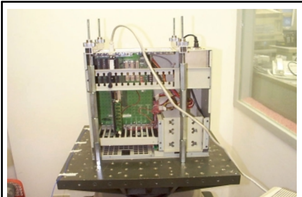
Y-Axis 1G random vibration test
