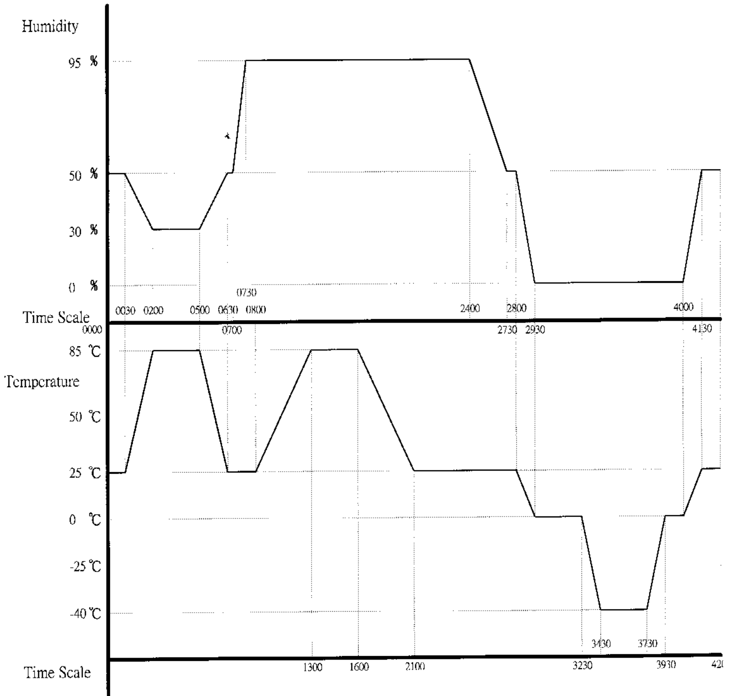
Temperature & Humidity Power ON/OFF Testing Curve :
