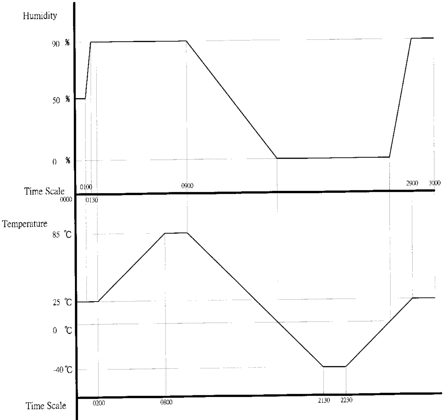
Temperature & Humidity Cycle Testing Curve :
