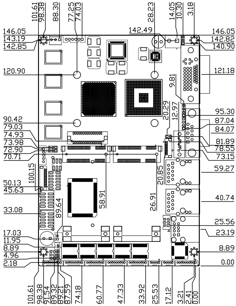
Component side
