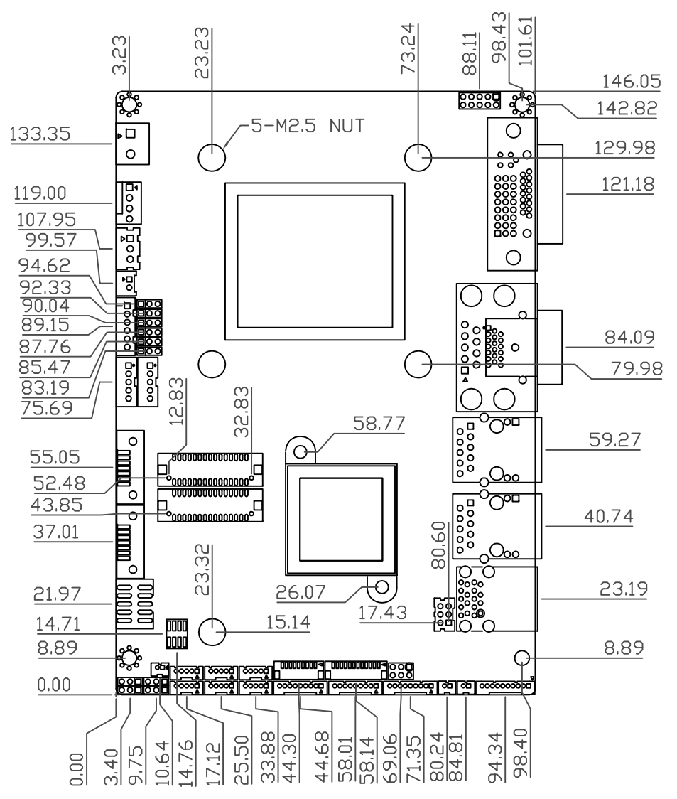
Component side
