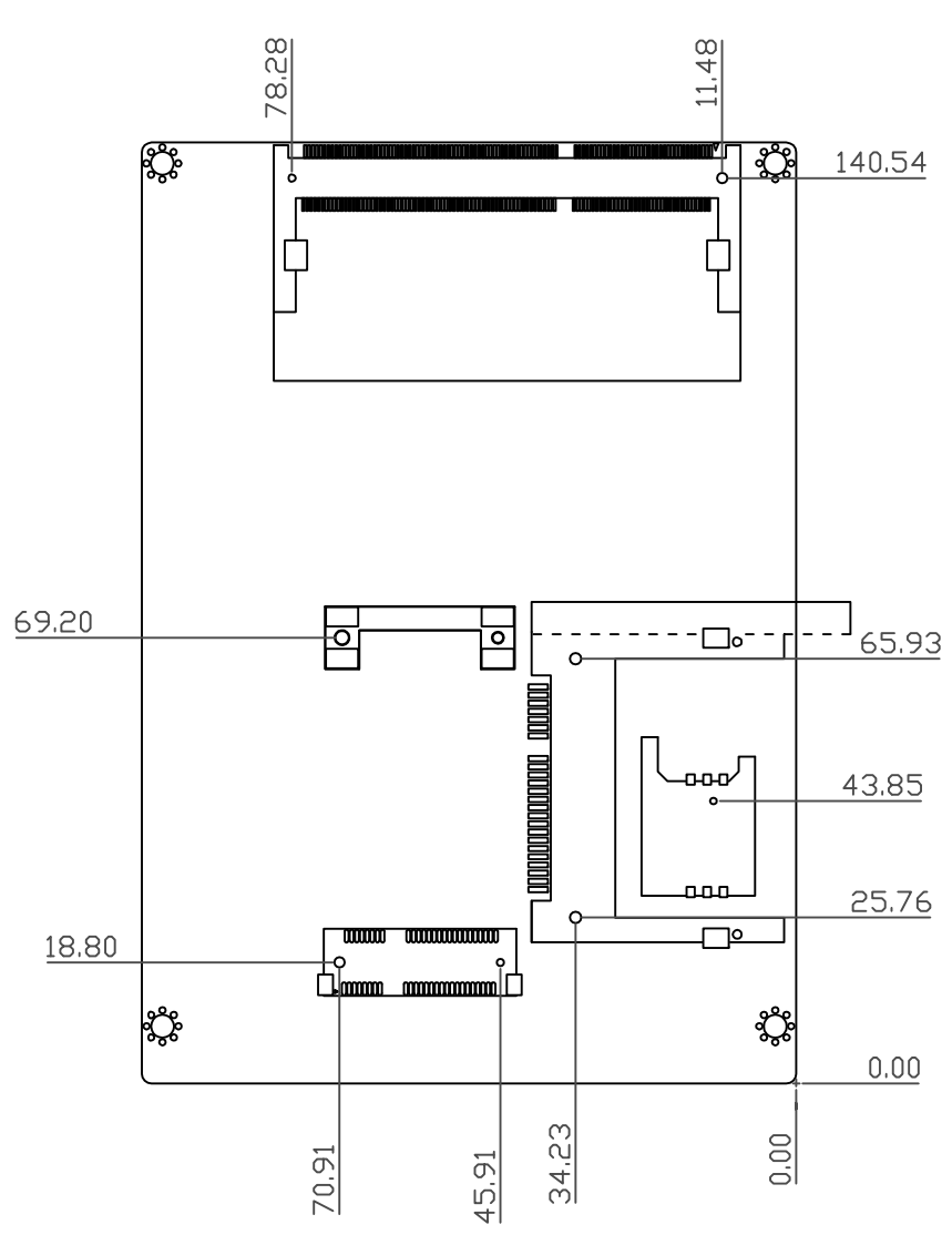
Solder side
