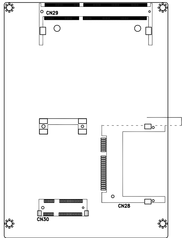
Solder side
