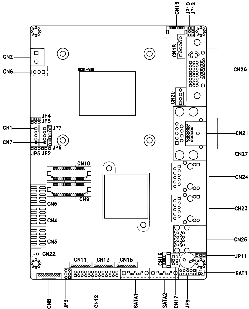
Component side
