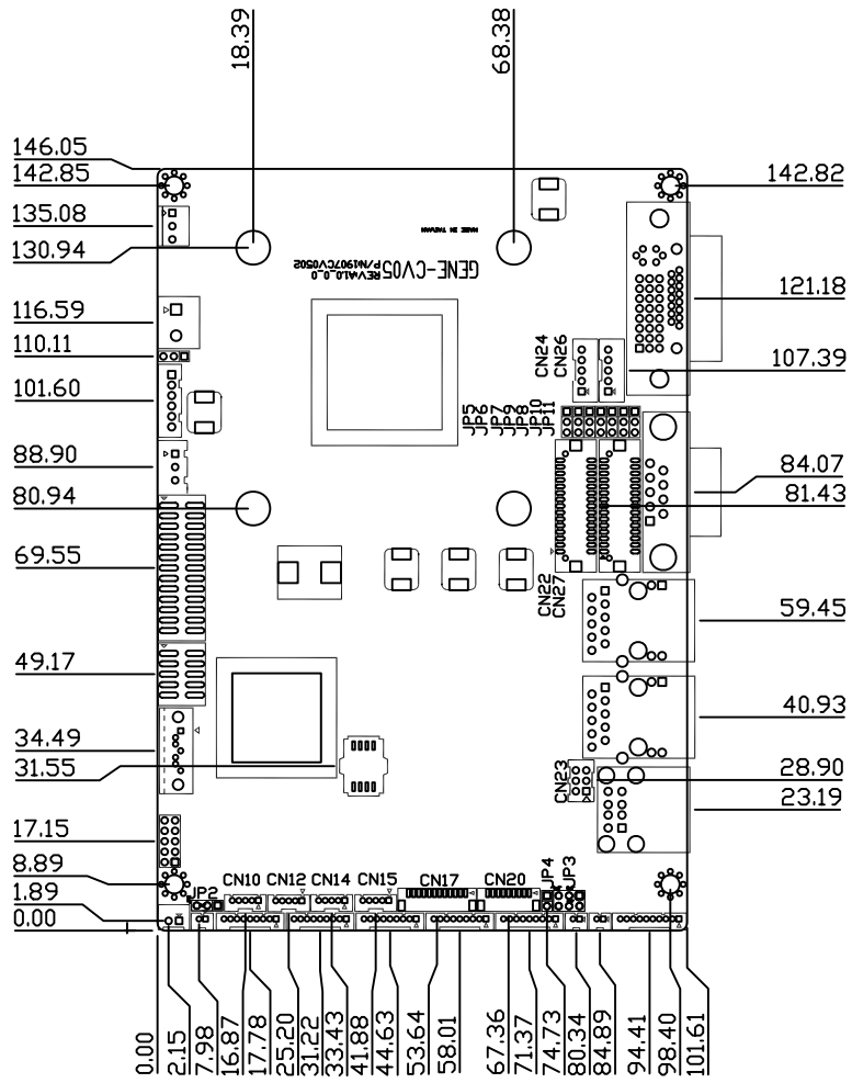
Component Side
