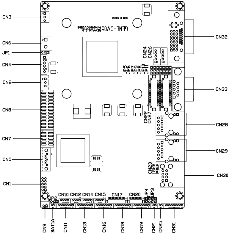
Component Side
