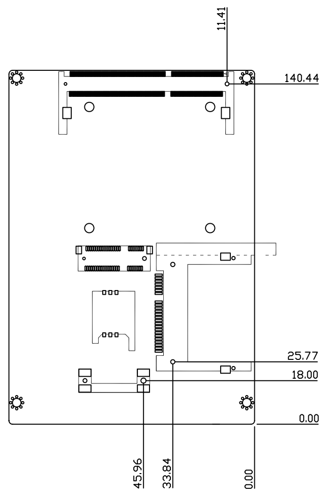
Solder Side
