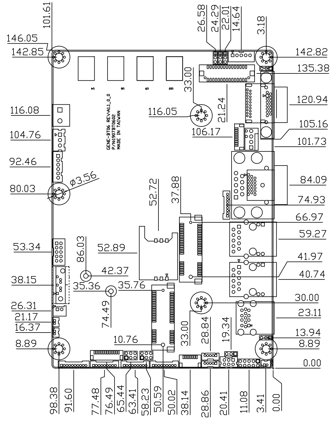
Component Side
