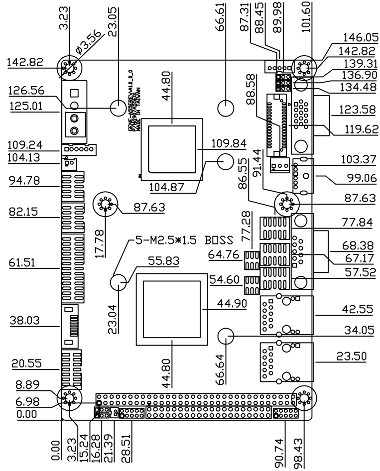
Component Side
