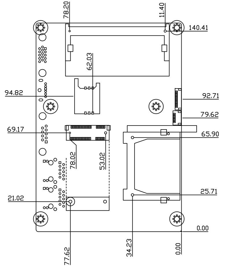
Solder Side
