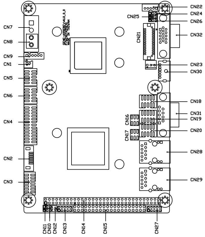
Component Side
