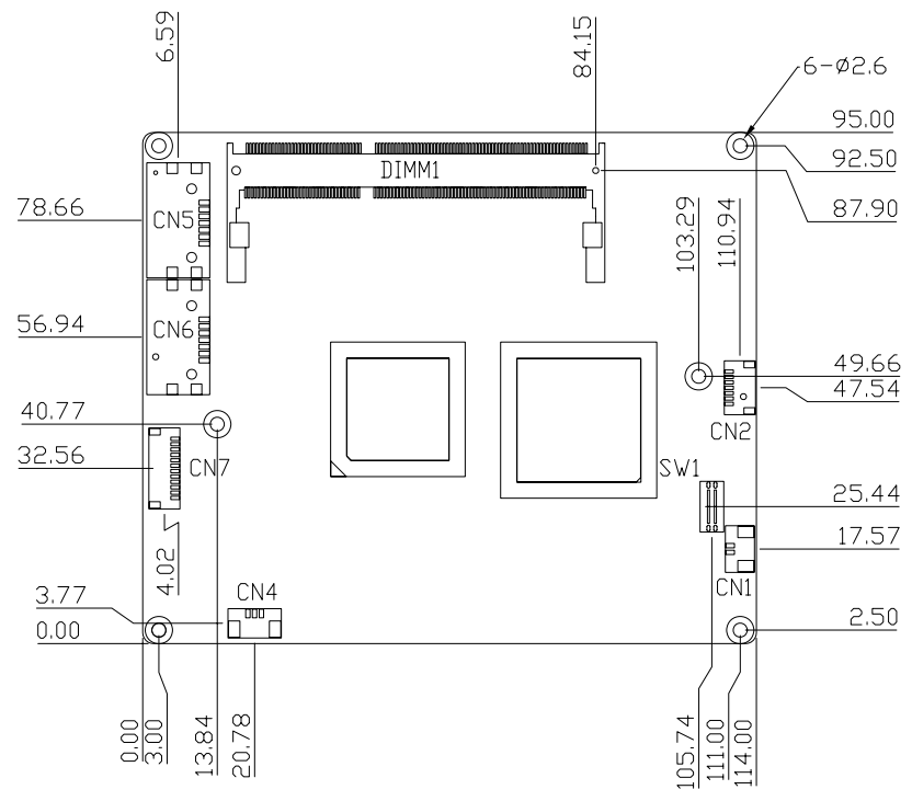
Component Side
