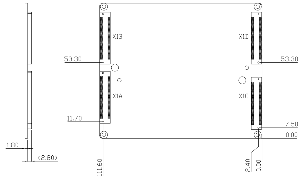
Solder Side
