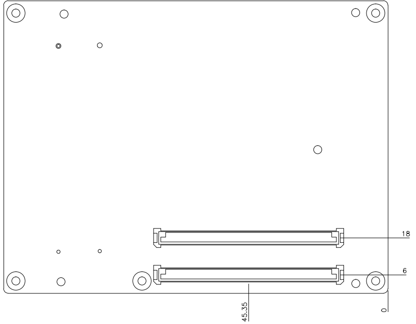
Solder Side
