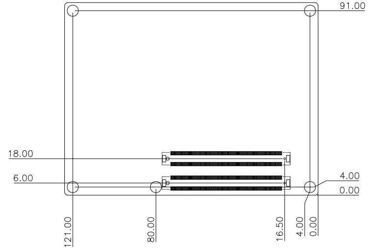
Solder Side
