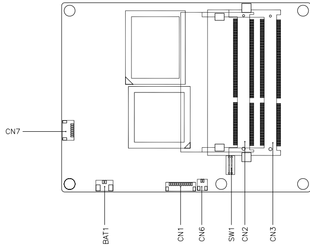
Component Side
