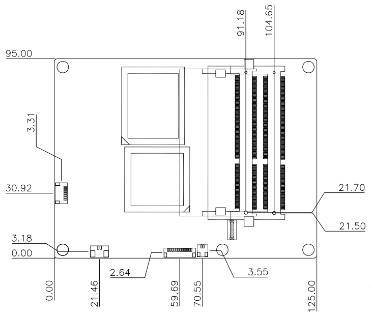
Component Side
