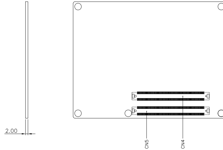
Solder Side
