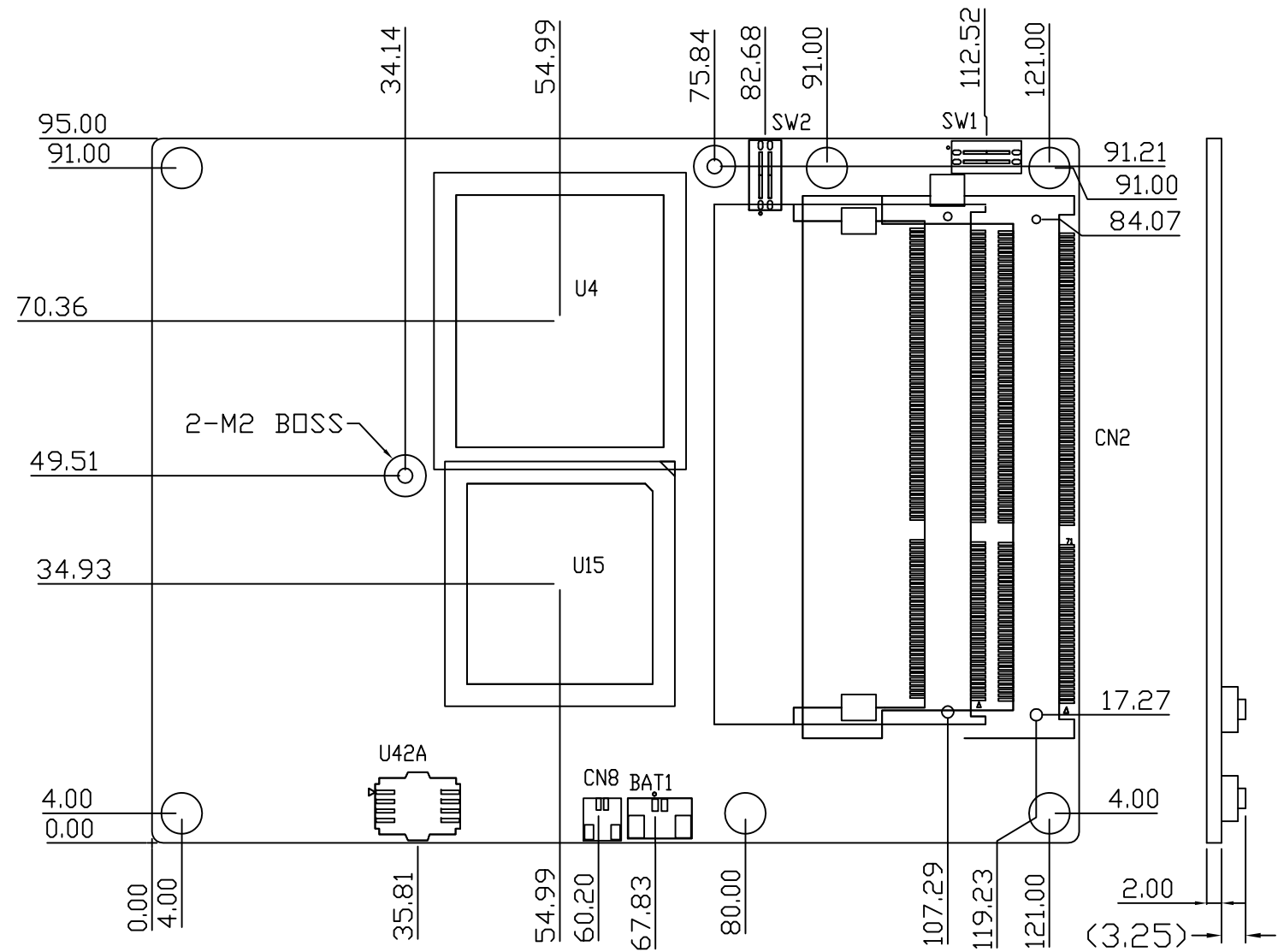
Component Side
