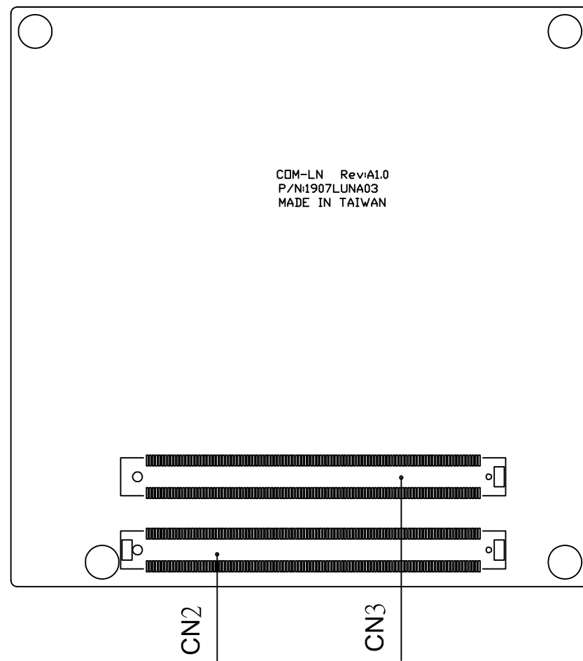
Solder Side
