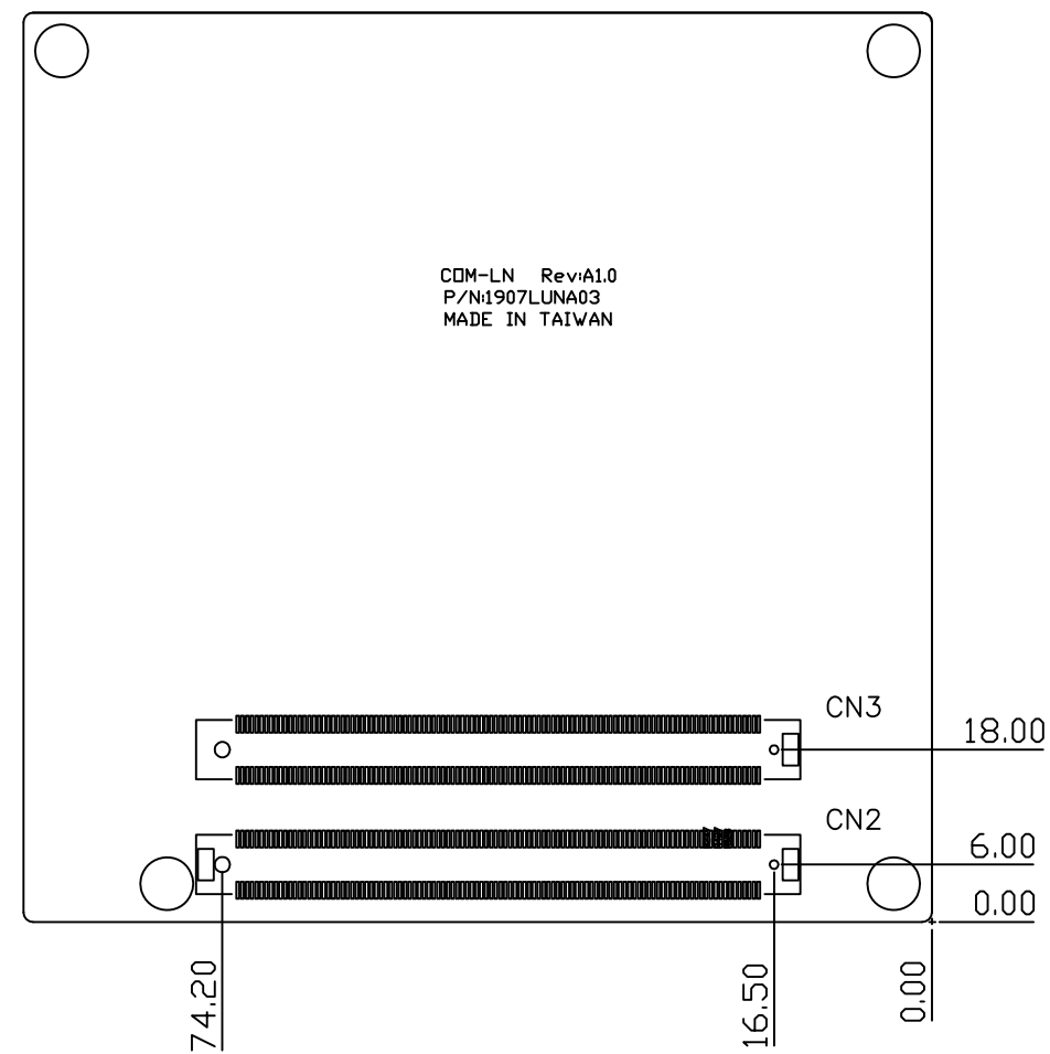
Solder Side
