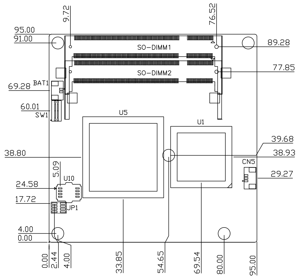
Component Side
