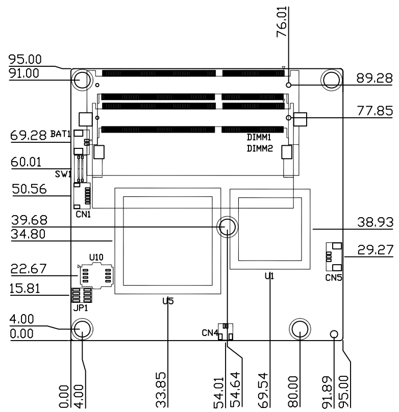
Component Side
