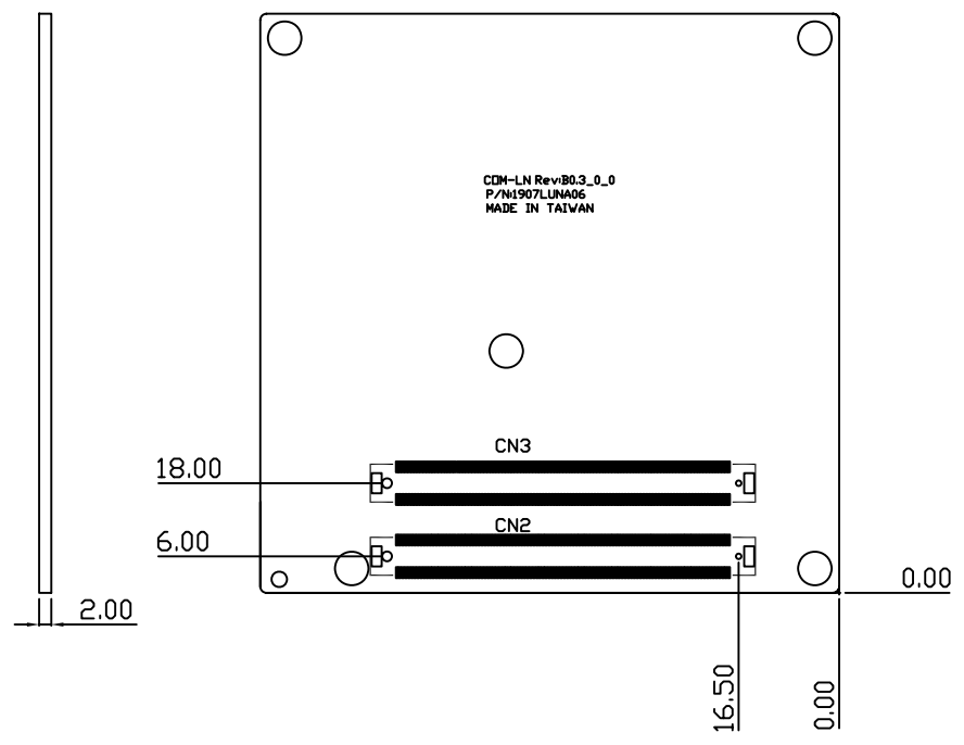
Solder Side
