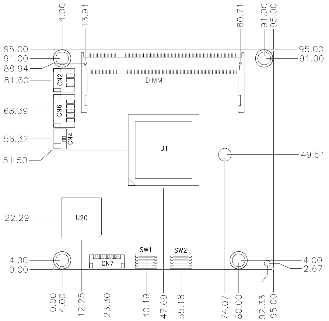
Component Side
