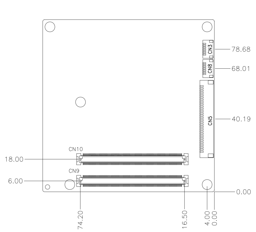
Solder Side
