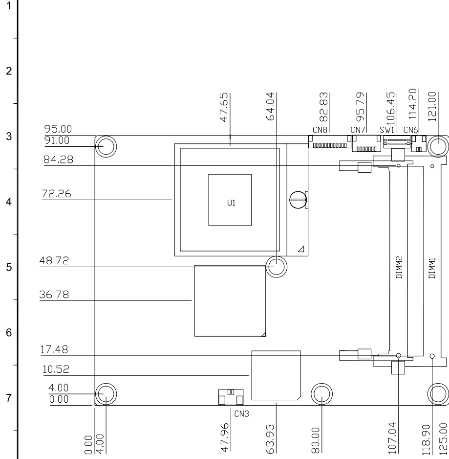
Component Side
