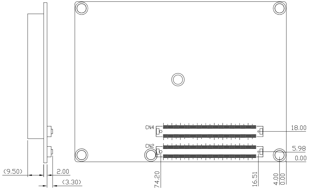
Solder Side
