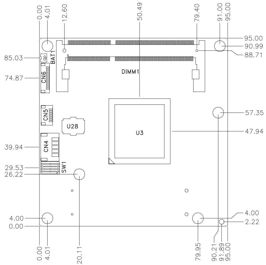
Component Side
