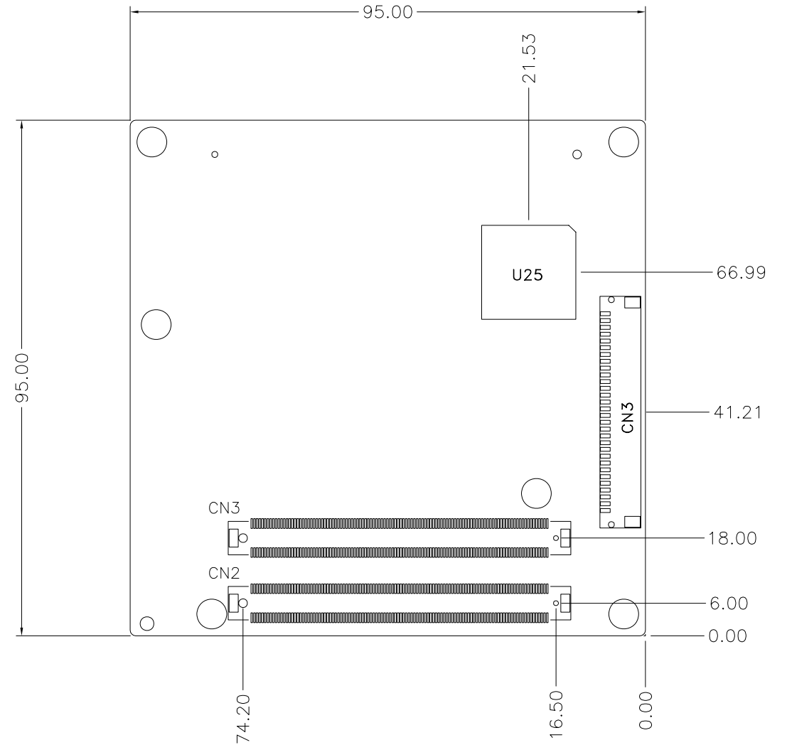
Solder Side
