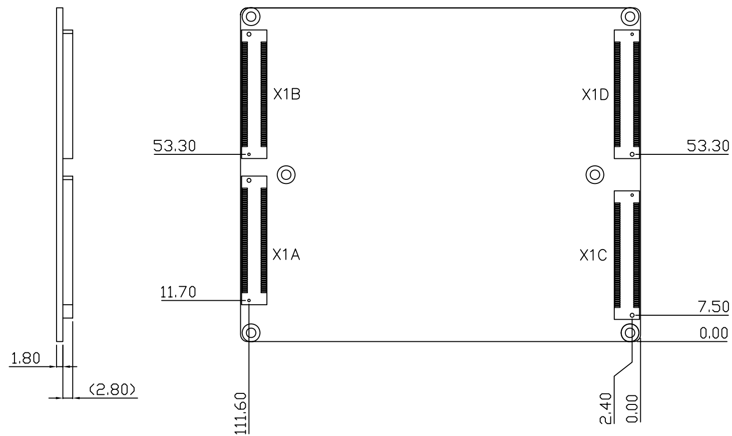
Solder Side
