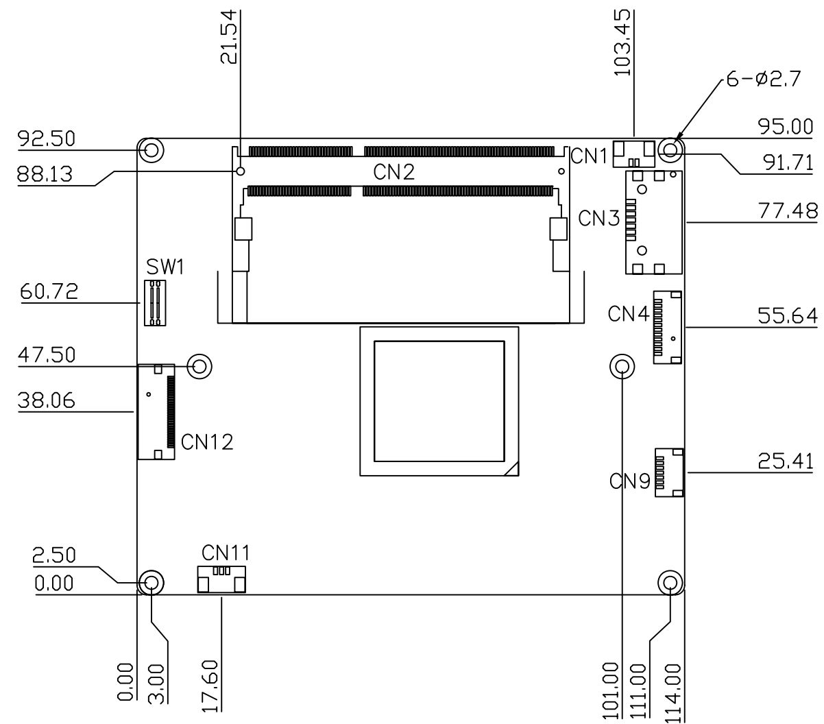
Component Side
