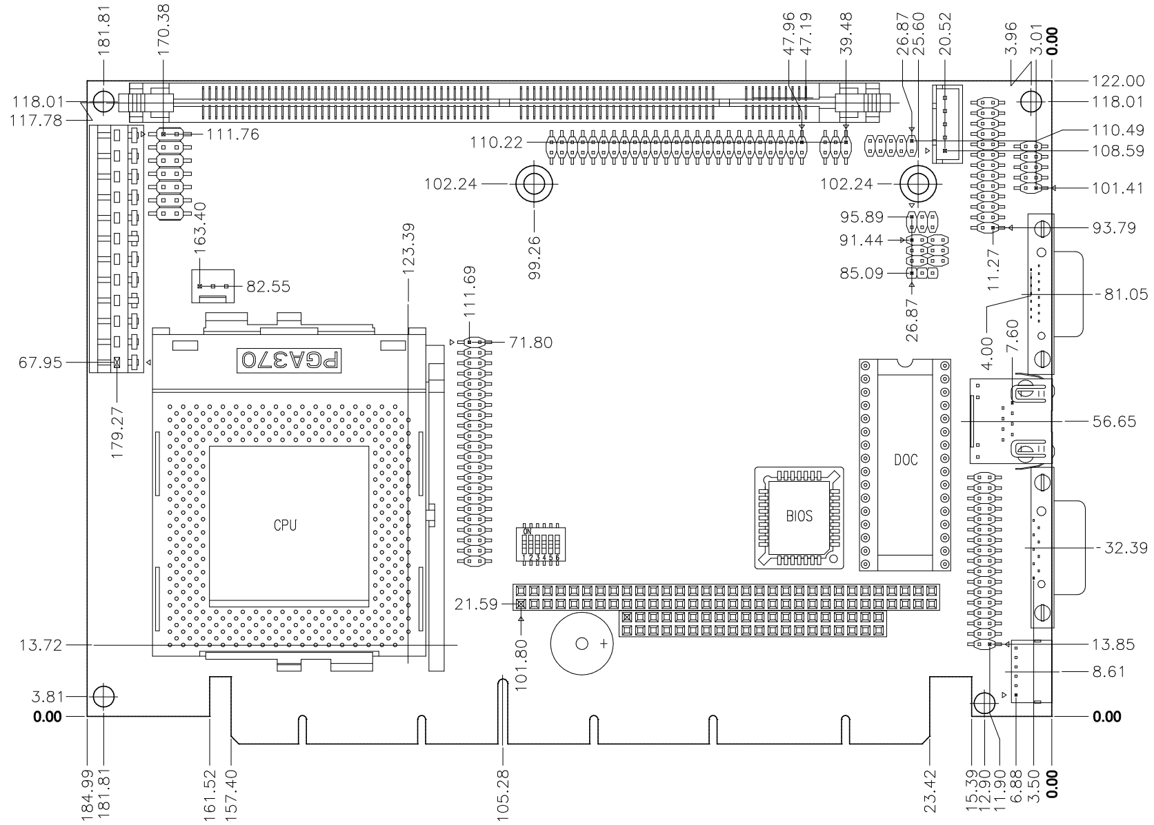
AAEON SBC-658 Rev A1.0 Mechanical Drawing UNIT:mm
