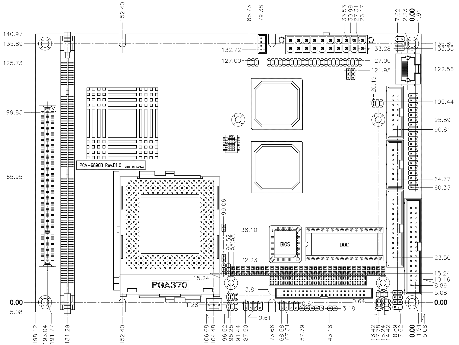
AAEON PCM-6890B Rev B1.0 Mechanical Drawing UNIT: mm
