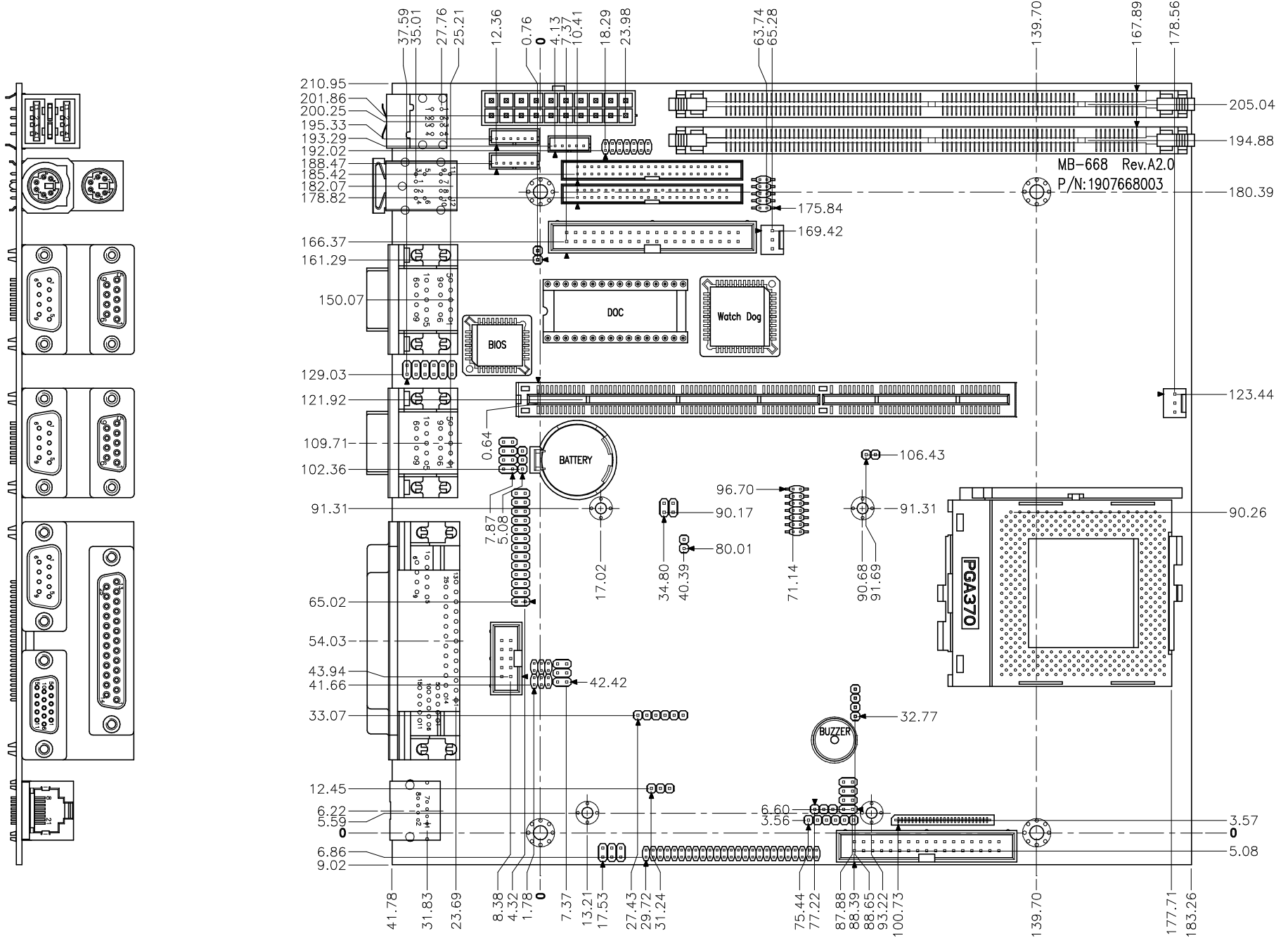
AAEON MB-668 Rev.A2.0 Mechanical Drawing UNIT: mm
