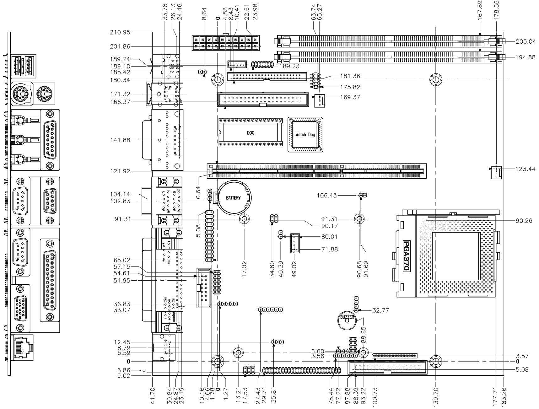
AAEON MB-662 Rev.A0 Mechanical Drawing UNIT: mm
