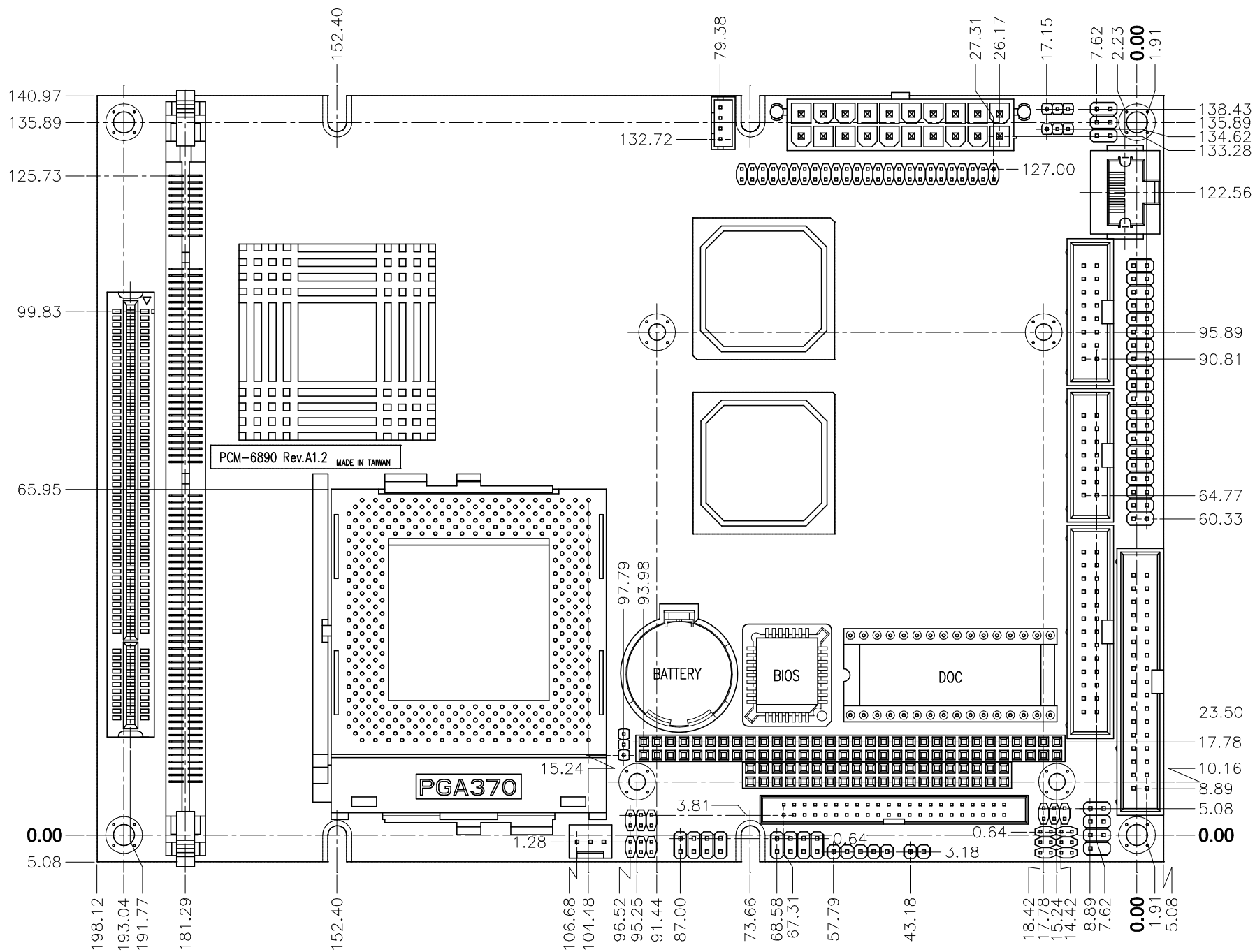
AAEON PCM-6890 Rev A1.2 Mechanical Drawing UNIT: mm
