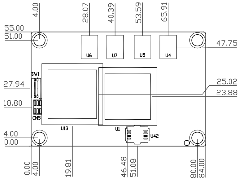
Component side
