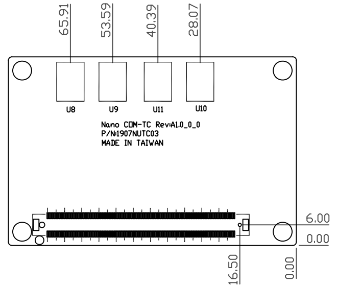
Solder side
