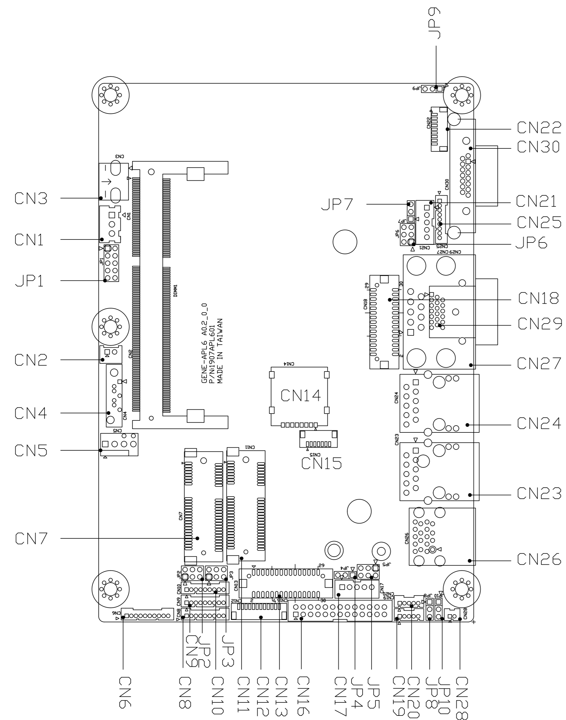
Component Side
