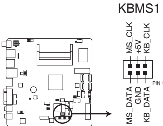
EMB-BT4 Series PS/2 keyboard/mouse connector
