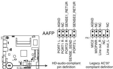
EMB-BT4 Front panel audio connector
