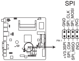
EMB-BT4 BIOS Programmable Connector
