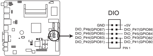
EMB-BT4 DIO connector
