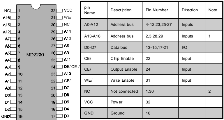
Figure1-MD2200 Pin-out
