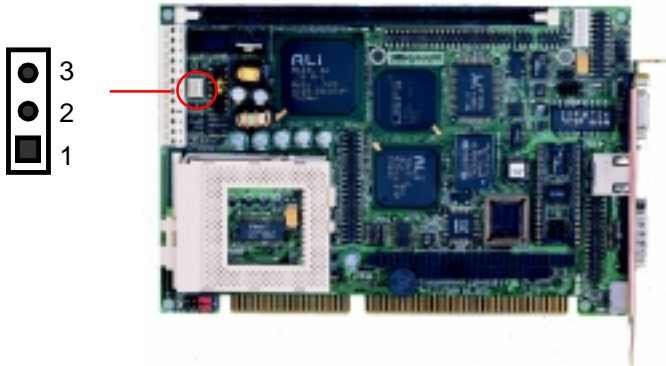
CPU fan power connector (CN4)
