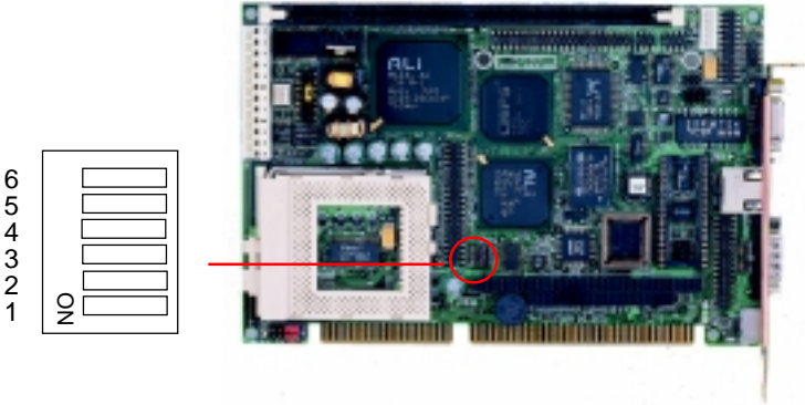
CPU clock select S2 (1 ~ 3)
