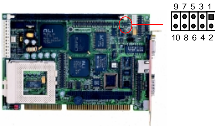
USB connector (CN7)
