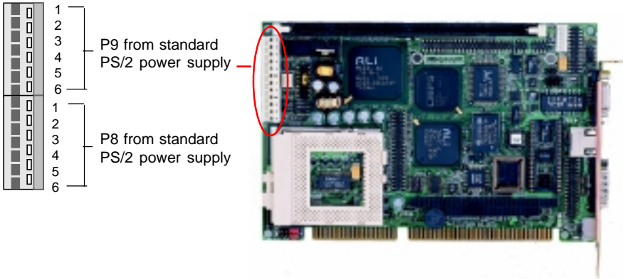
Power connector pin assignments (PWR1)
