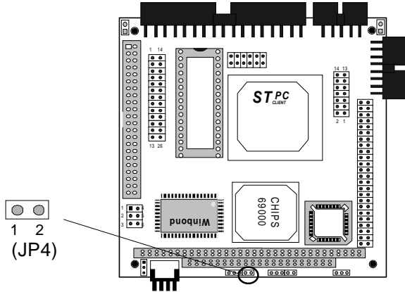
Keyboard lock function (JP4)
