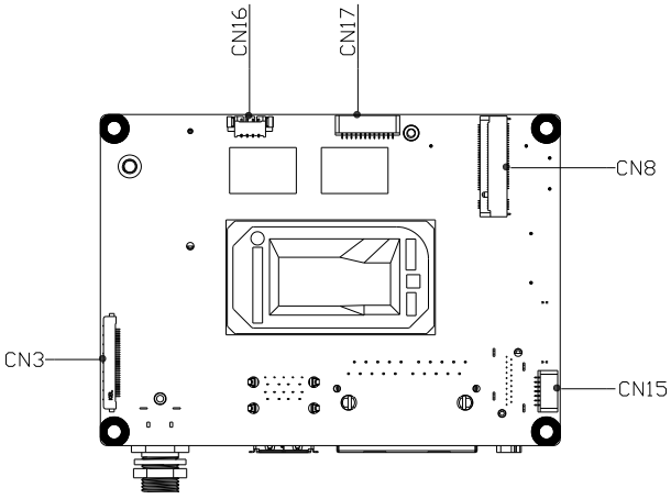
Solder Side
