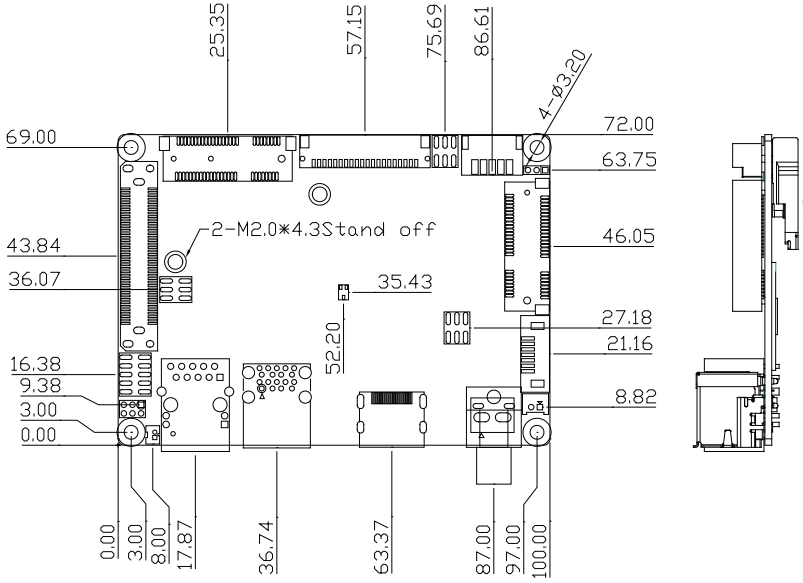
Component Side
