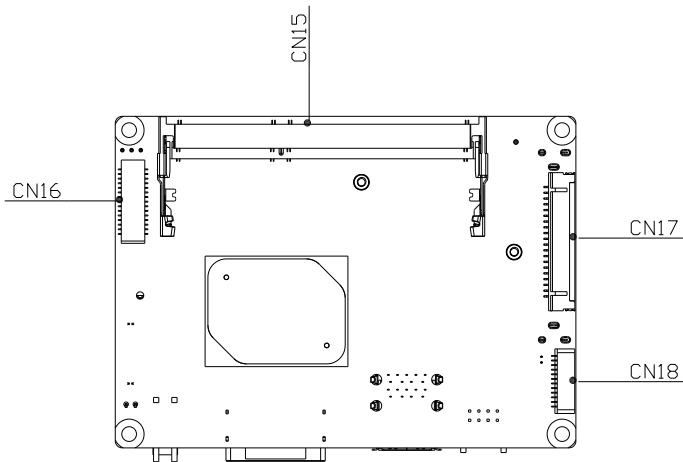
Component Side
