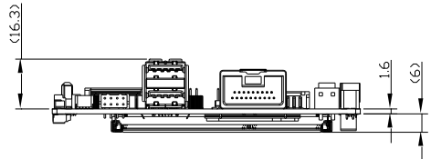
Component Side
