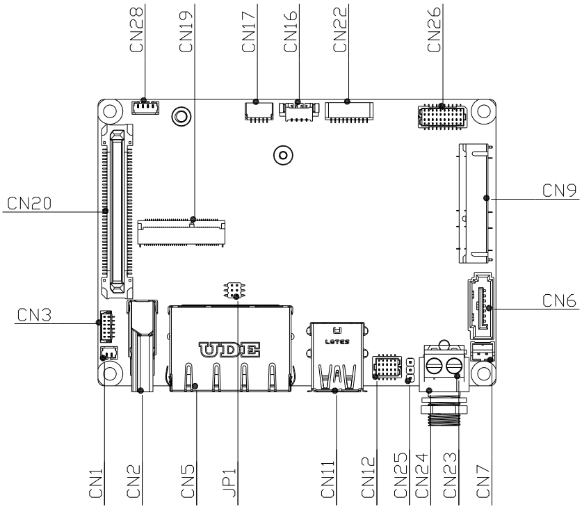
Component Side
