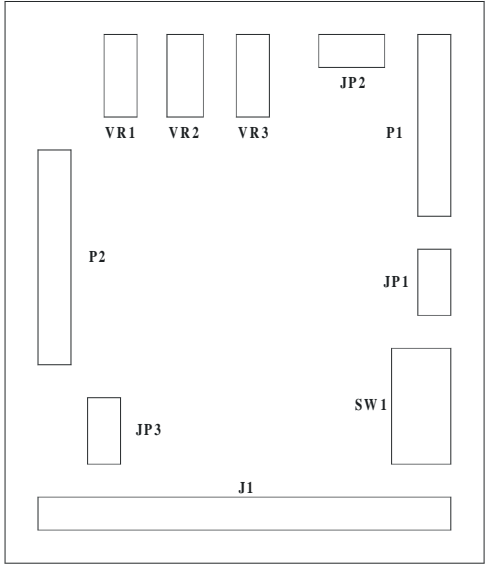
Connectors, switches and VR locations
