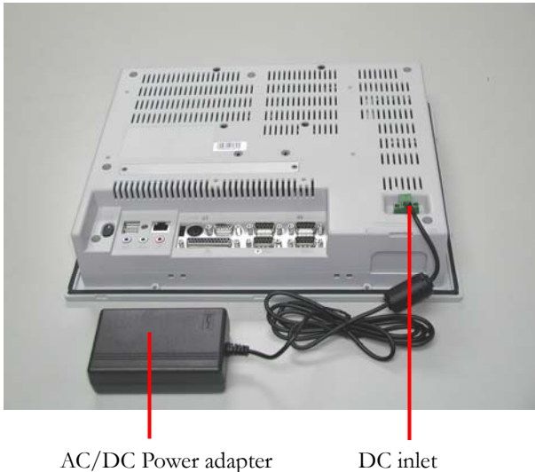
Figure 2.5: Connect the power cord to the DC inlet
