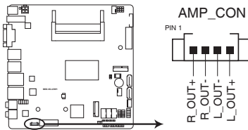
MIX-KLUW1 Audio stere. output with Amp connector
