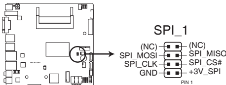
MIX-KLUW1 BIOS programmable connector
