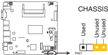
MIX-KLUW1 Chassis intrusion connector
