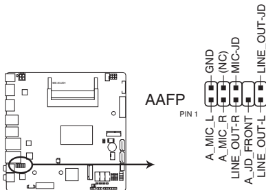
MIX-KLUD1 Front panel audio connector
