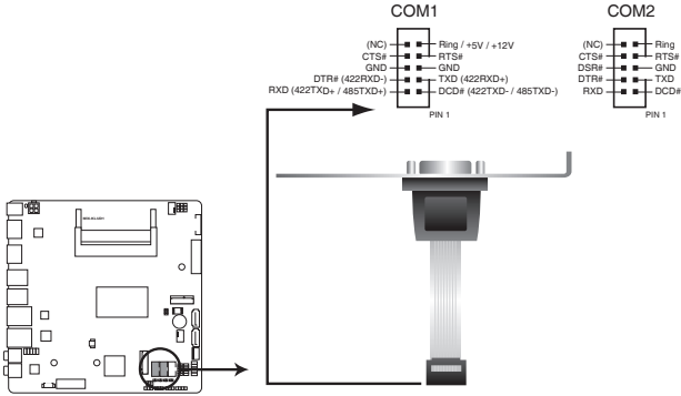
MIX-KLUD1 Serial port connectors
