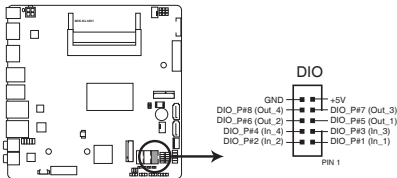
MIX-KLUD1 Digital I/O connector
