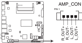
MIX-KLUD1 Audio stere. output with Amp connector
