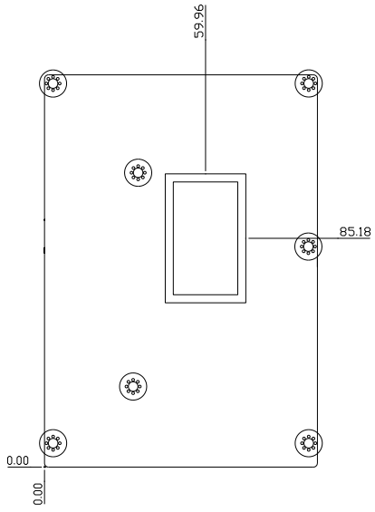
Solder Side
