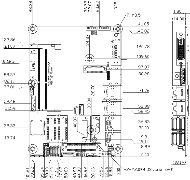
Component Side
